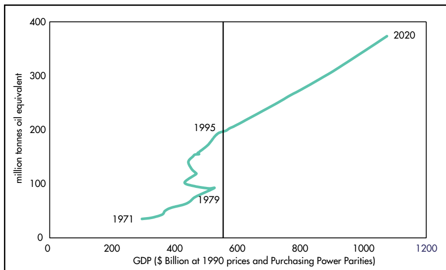
Figure 20.1: Total Final Energy Consumption versus GDP (1971 - 2020)
